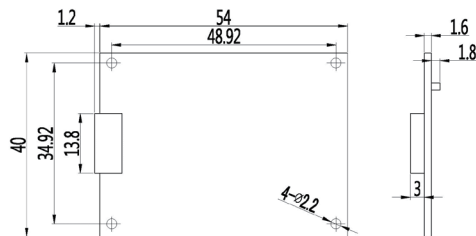
main board (unit: mm)
