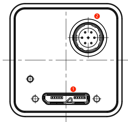
Figure 8- 9 USB interface uncooled camera
