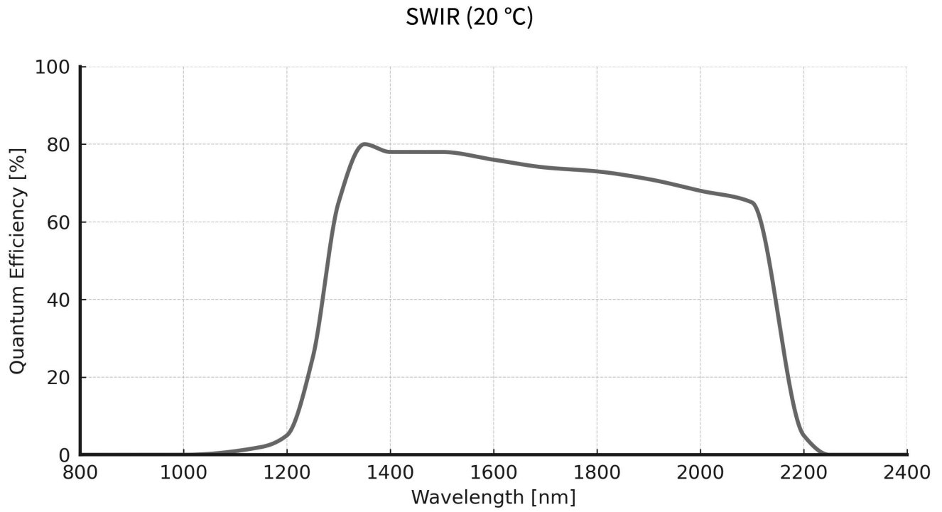
Figure 5- 3 EHD333KMB-E1222 QE Curve
