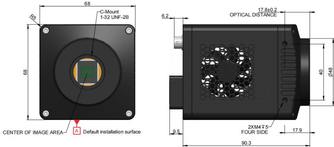
Figure 8- 20 The Front and side view dimensions of the GigE interface camera
