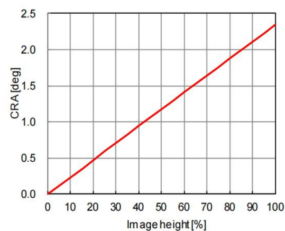
Figure 7- 5 IMX990 CRA characteristics
