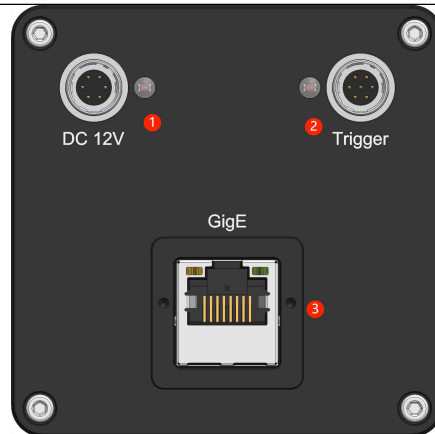
Figure 8- 17 GigE interface refrigerated camera
