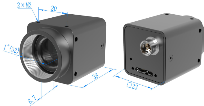
Figure 8- 4 USB interface uncooled camera dimensions
