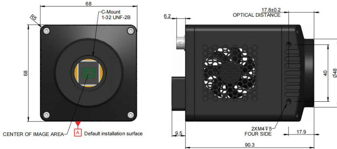
Figure 8- 10 The Front and side view dimensions of the GigE interface camera
