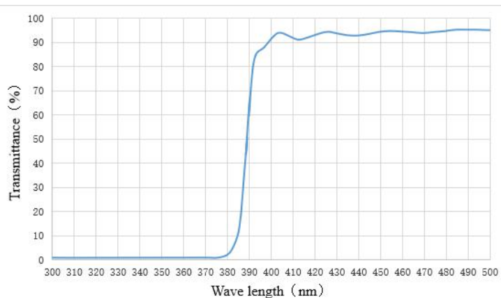
Figure 7- 6 Long wave pass filter LPF390H transmittance curve
