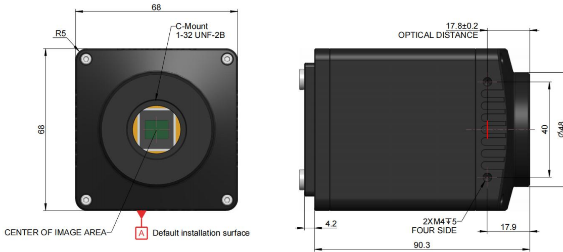
Figure 8- 11 The Front and side view dimensions of the USB interface camera
