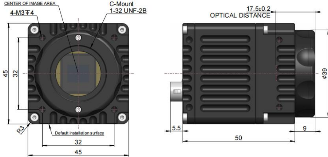
Figure 8-12 GigE/USB interface compact camera form factor
