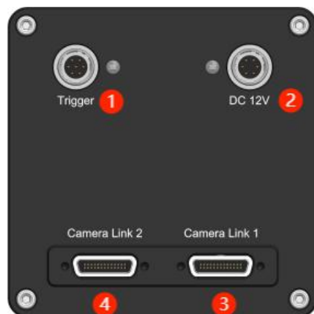
Figure 8- 8 CL interface refrigerated camera
