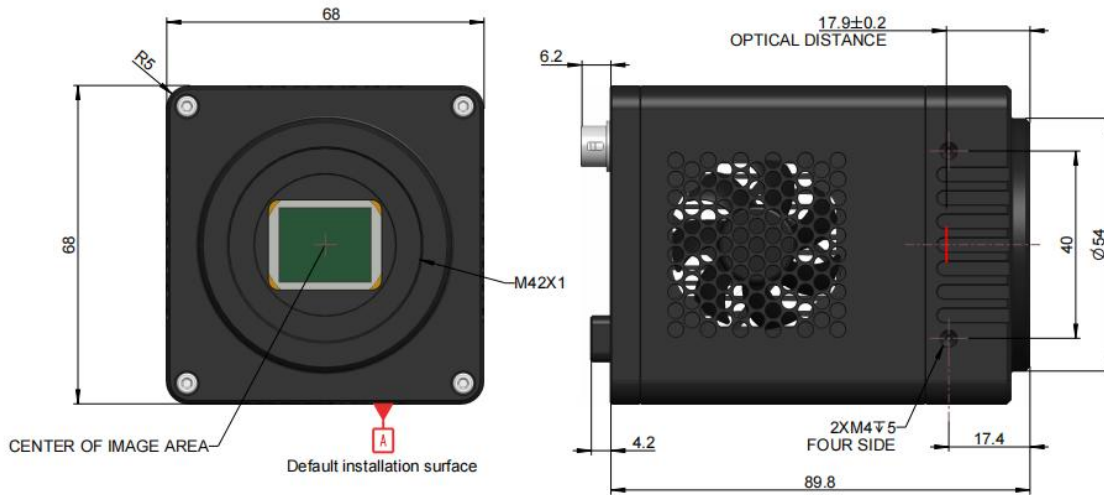
Figure 8-13 The Front and side view dimensions of the CL interface camera
