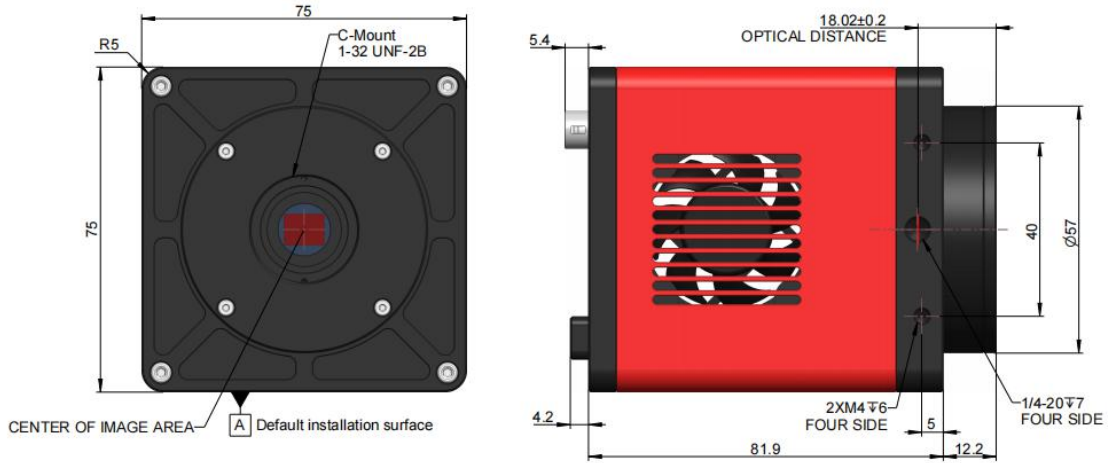
Figure 8- 3 CL interface refrigerated camera dimensions
