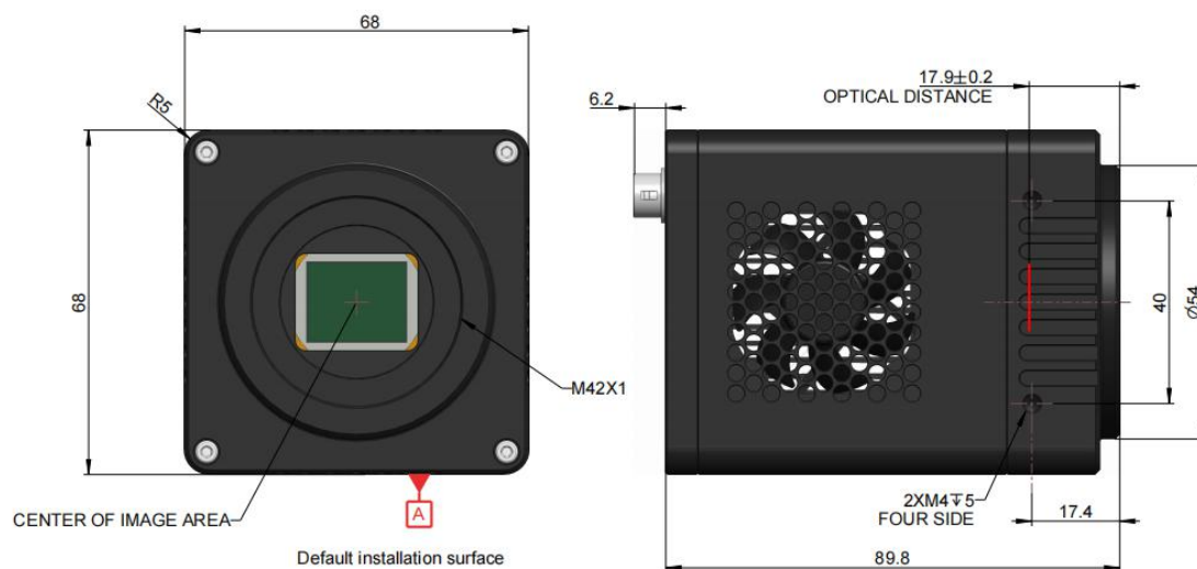
Figure 8- 15 The Front and side view dimensions of the USB interface camera
