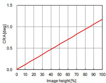
Figure 7- 4 IMX991 CRA characteristics
