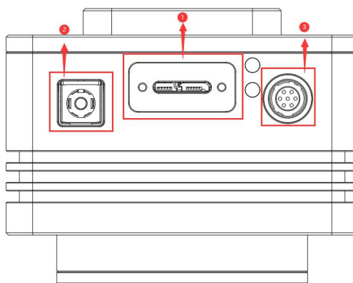
Figure 8- 6 USB interface refrigerated camera
