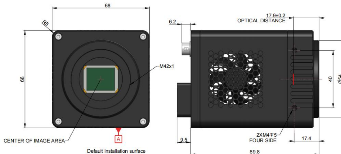
Figure 8- 14 The Front and side view dimensions of the GigE interface camera
