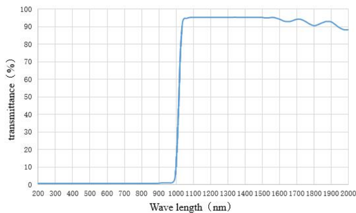
Figure 7- 7 Long wave pass filter LP1000H transmittance curve
