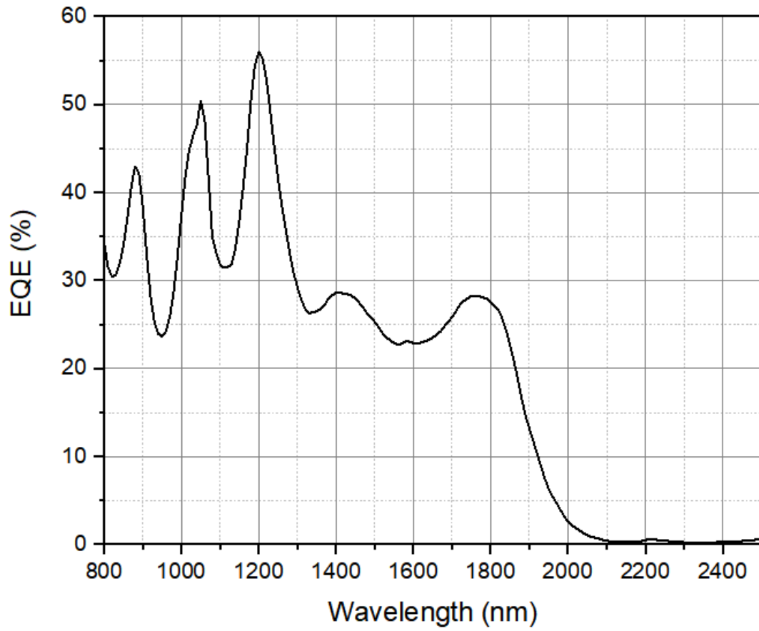
Figure 6-1 MaxCam-640TE-817CQD QE Curve
