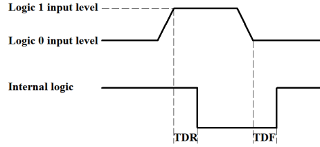
Figure 10-2 Input logic levels
