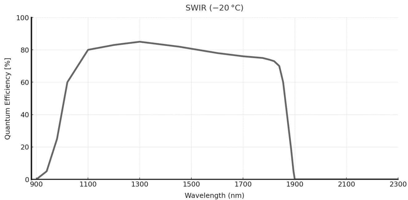
Figure 5-2 5.1.6 MaxCam-640TE-1900 QE Curve
