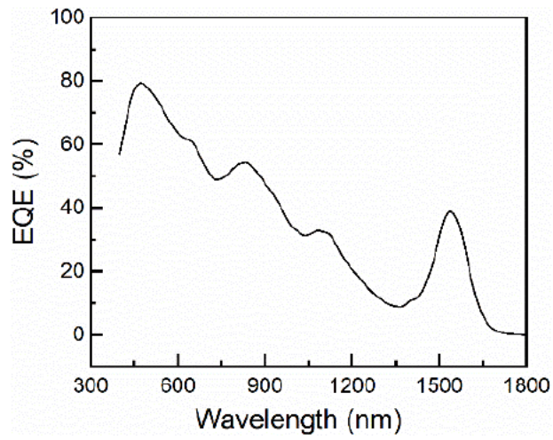
Figure 6-2 MaxCam-640TE-417CQD-U200 QE Curve
