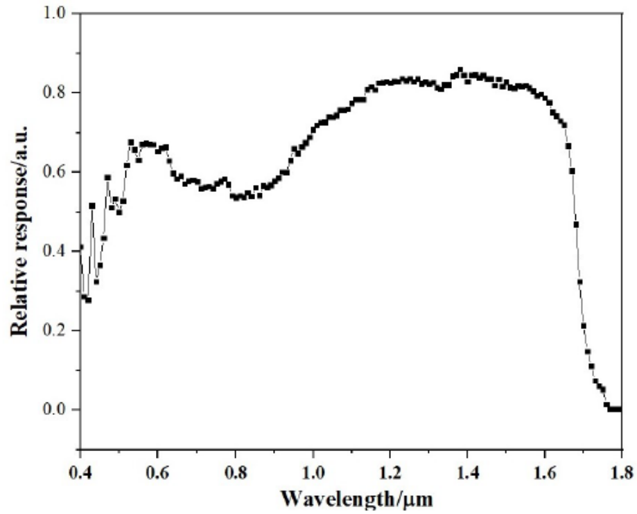
Figure 6 1 MaxCam-1280 QE Curve
