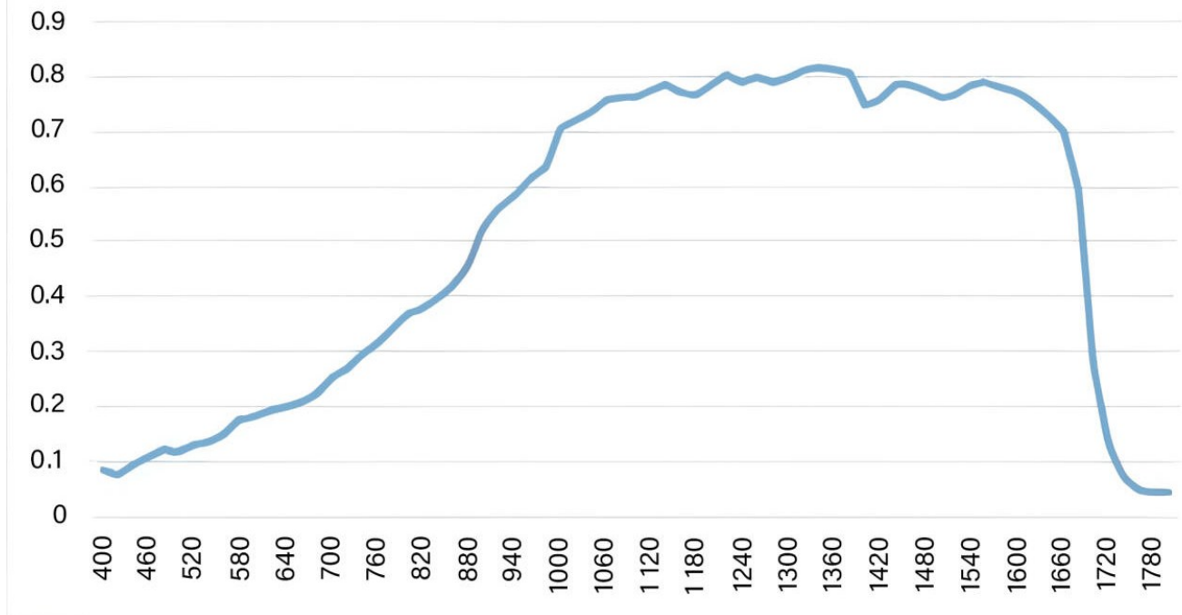
Figure 5-1 MaxCam-640TE417 QE Curve
