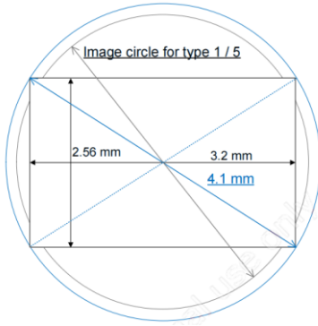
Figure 7-2 IMX991 relationship between image circle and pixel area
