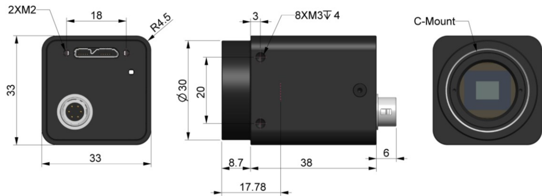
Figure 8-5 SC-Series USB interface uncooled camera
