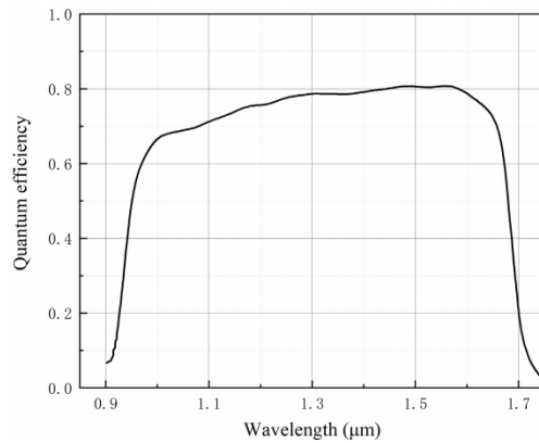
Figure 4-1 MaxCam-1280 QE Curve
