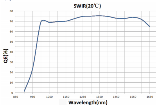
Figure 4-2 MaxCam-640 QE Curve
