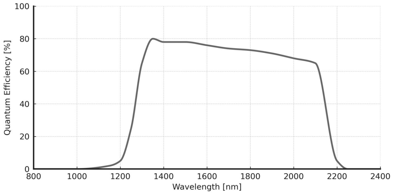
Figure 5-3 MaxCam-640TE-2200-U270 QE Curve
