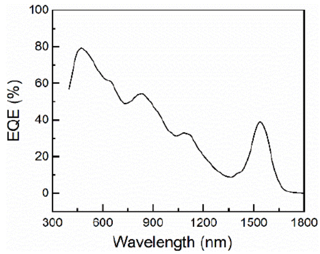
Figure 6-3 SC640TR-1700CQD-UMV QE Curve
