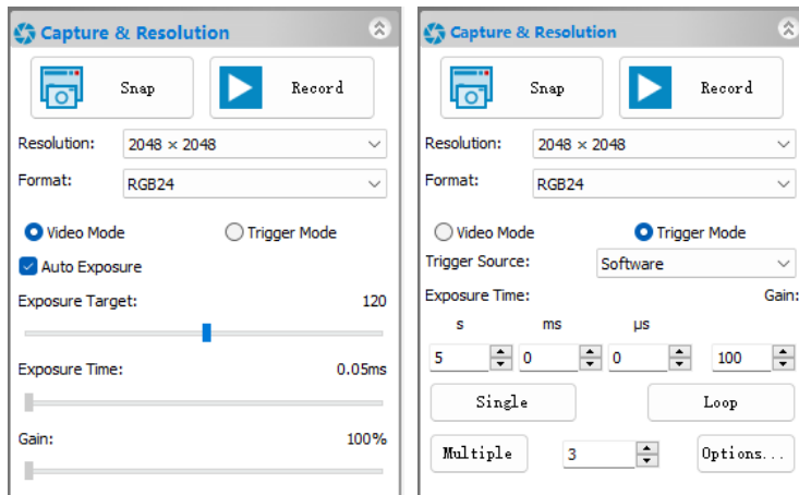
Figure 11-3 Video Mode and Trigger Mode on the Capture & Resolution group in ToupView
