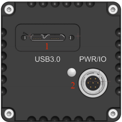
Figure 8-23 SC1280TR-UMV USB interface small size camera
