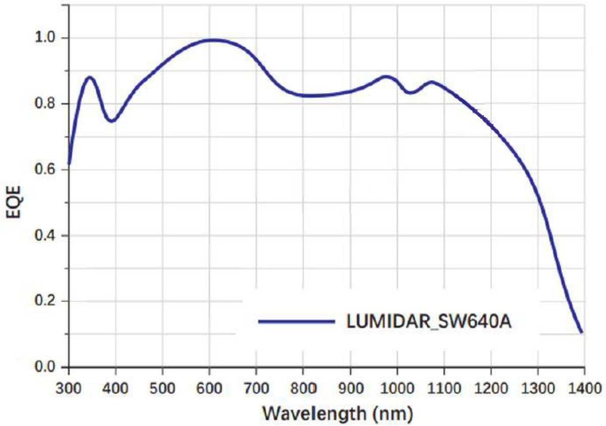
Figure 6-4 SC640TR-1400CQD-UMV QE Curve
