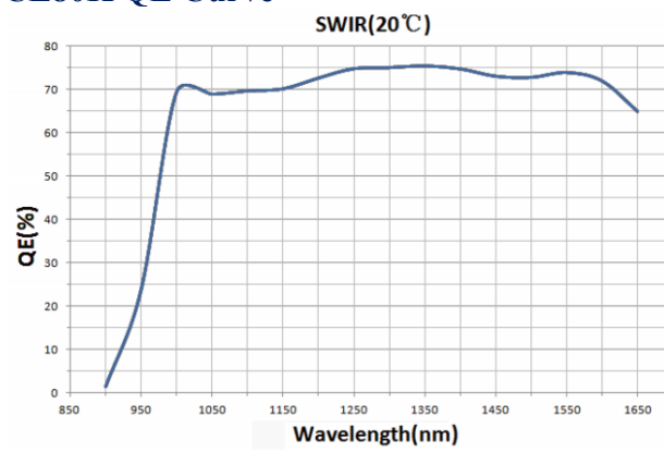
Figure 4-3 MaxCam-2048TE-CL80K QE Curve
