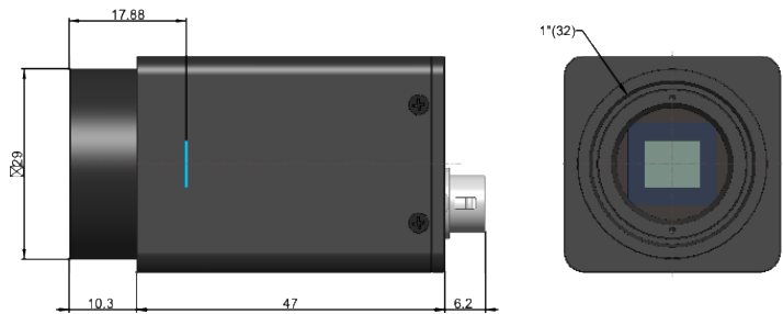
Figure 8-6 SC-Series GIG interface uncooled camera dimensions
