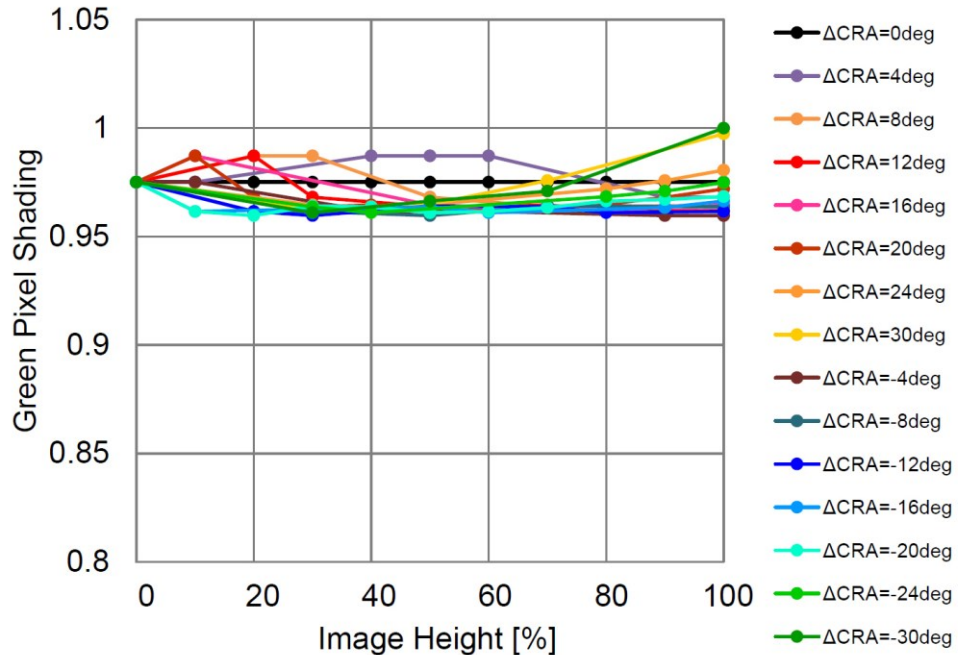
\Delta CRA - G Shading characteristics at Horizontal angle
